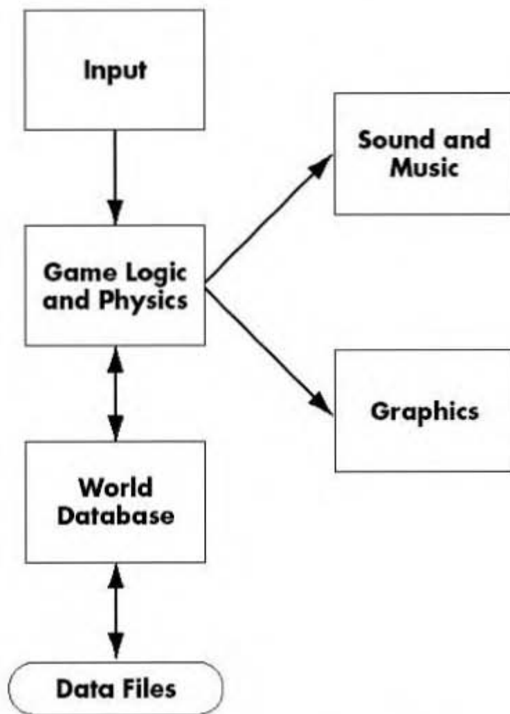
Figure 1.1 A game is composed of various subsystems.
