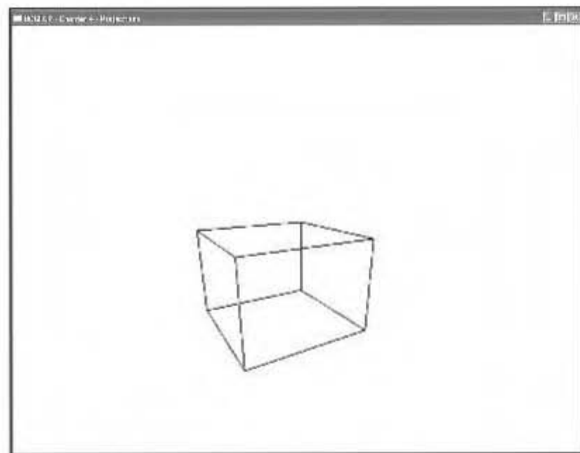
Figure 4.16 Perspective projection.
