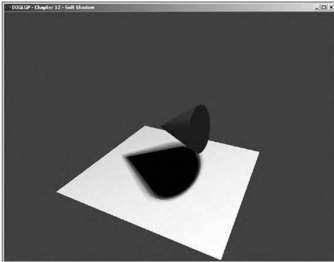
Figure 12.4 Soft shadows.
