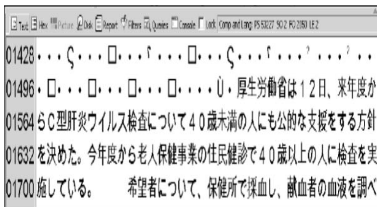
Figure 1.5 Foreign-language forensics.
