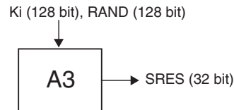
Figure 6.3: GSM SRES Generation
