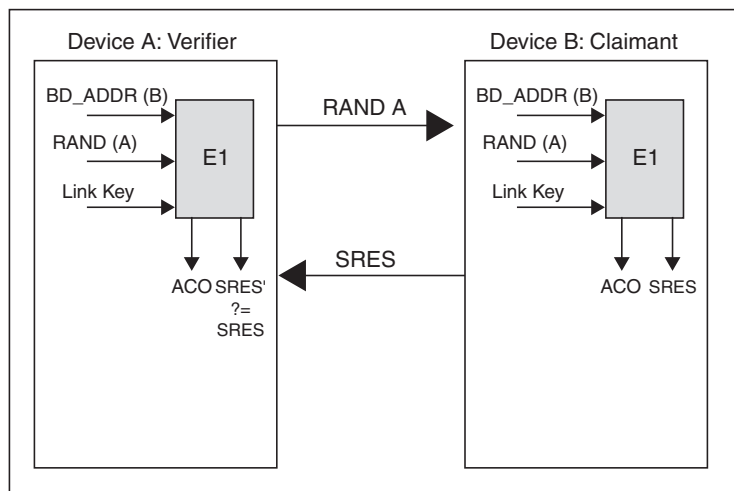
Figure 8.6: Bluetooth Authentication
