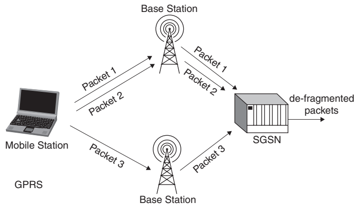
Figure 6.6: GPRS Roaming
