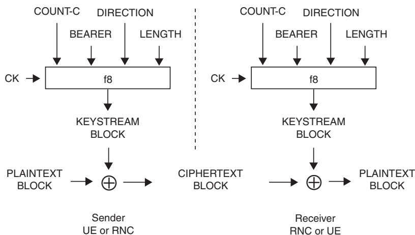
Figure 6.12: UMTS Encryption
