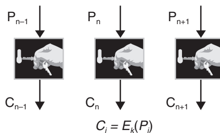
Figure 1.12: ECB Mode
