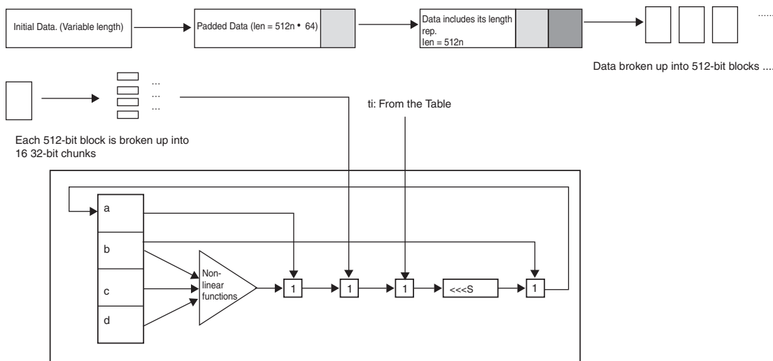
Figure 2.26: MD5
