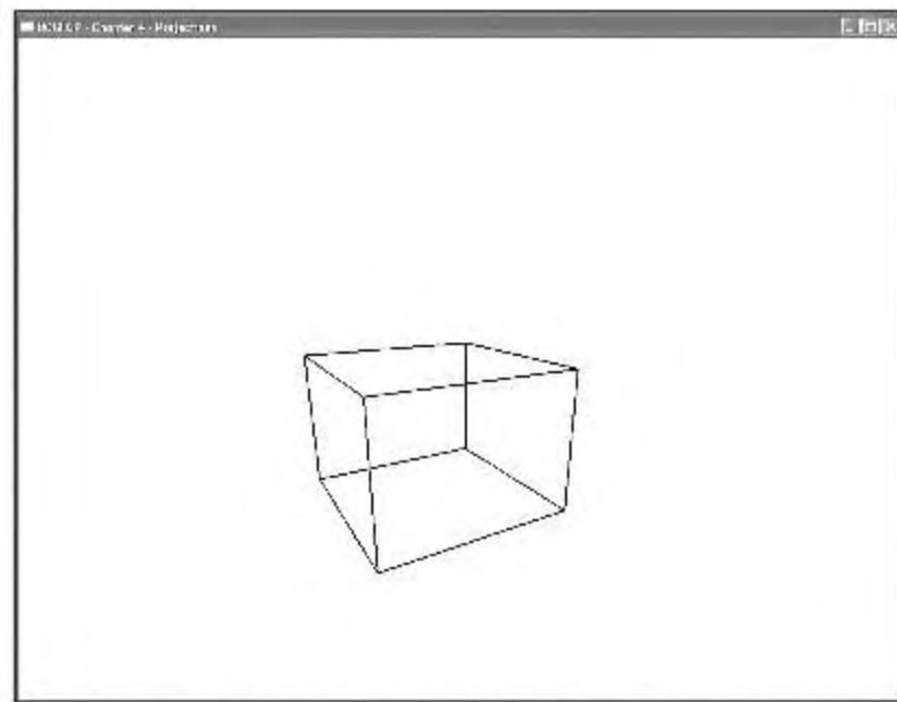
Figure 4.16 Perspective projection.
