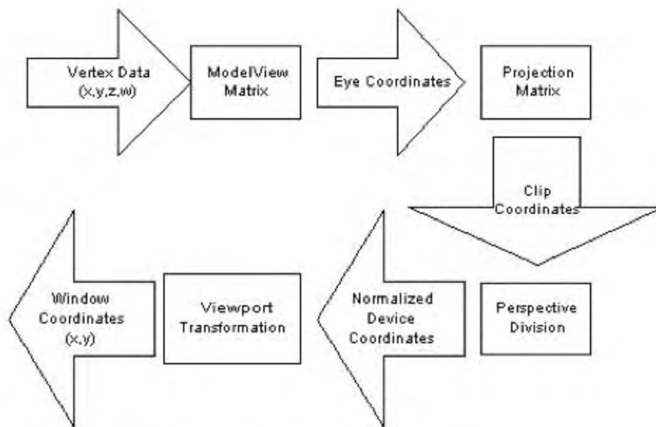
Figure 4.1 The vertex transformation pipeline.
