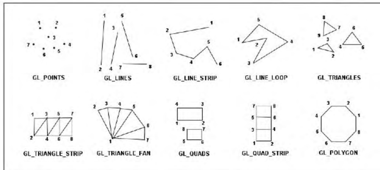
Figure 3.1 OpenGL primitive types.
