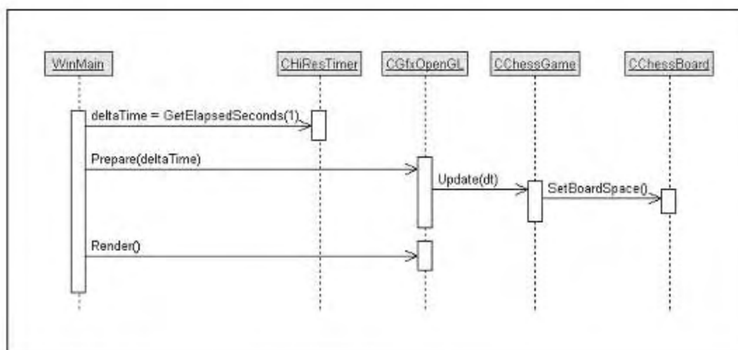
Figure 13.3 Update sequence diagram.
