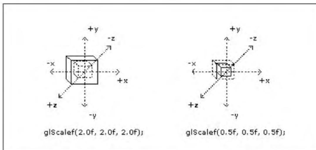
Figure 4.10 The glScale() function.
