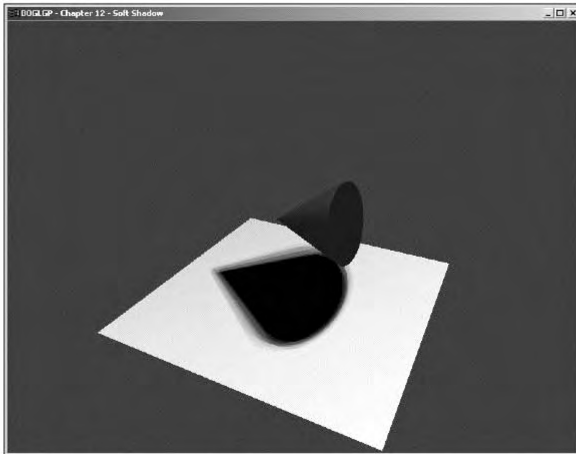
Figure 12.4 Soft shadows.
