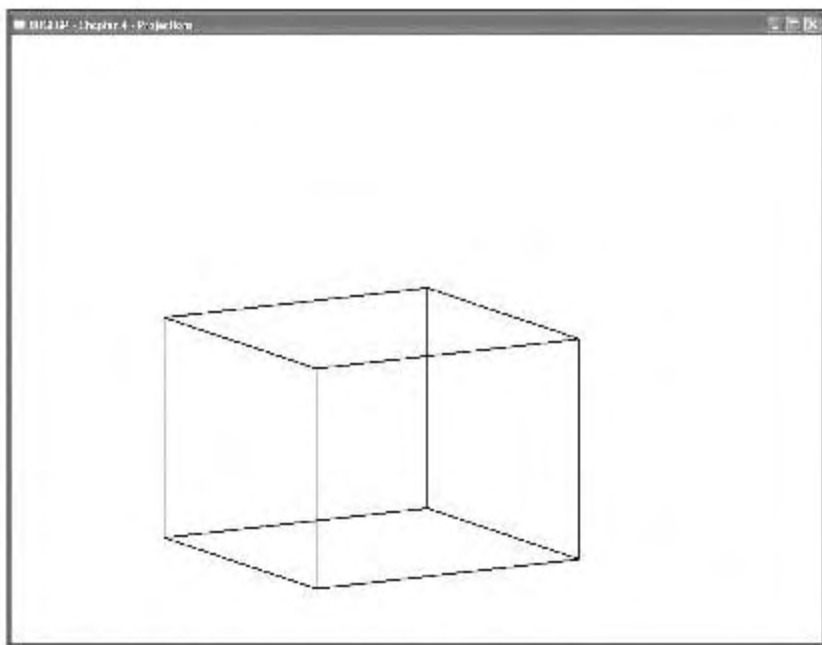
Figure 4.15 Orthographic projection.
