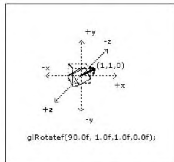
Figure 4.8 Rotation about an arbitrary axis.
