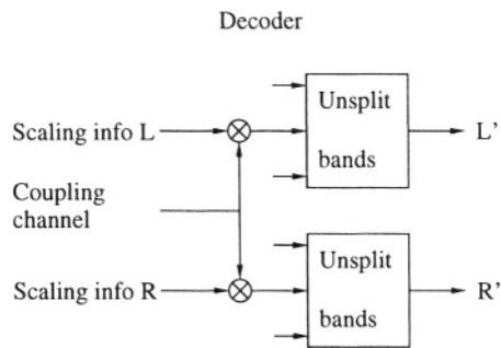
Figure 11.12 Diagram of an intensity stereo decoder.
