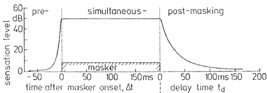
Figure 11.2 Temporal masking threshold (from [15]).
