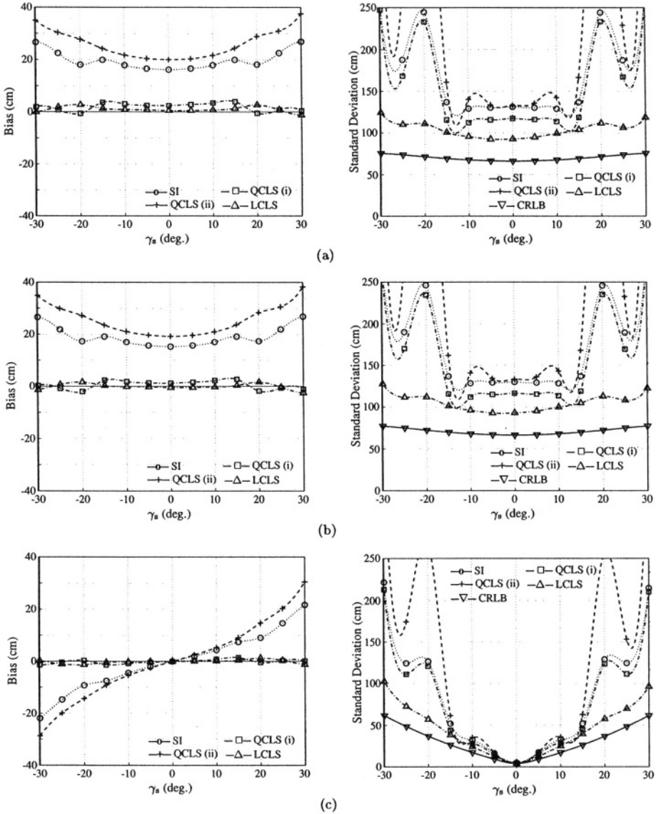
Figure 9.5 Comparisons of empirical bias and standard deviation among the SI, QCLS-i, QCLS-ii, and LCLS estimators with zero mean colored Gaussian errors of standard deviation \sigma_\epsilon = 1 cm. (a) Estimators of x_s , (b) estimators of y_s , (c) estimators of z_s .
