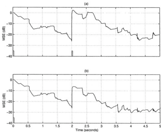
Figure 7.5 . Effects of echo path changes in terms of mean-square error of the two-channel robust frequency-domain algorithm with the pseudo-coherence-based DTD (no double-talk present). The echo paths in the receiving room change as: (a) Time delay of 5 samples at 2 s. (b) 6-dB increase of echo path gain at 2 s. The rectangles in the bottom of the figures indicate where double-talk has been detected (in this case, they are false alarms).
