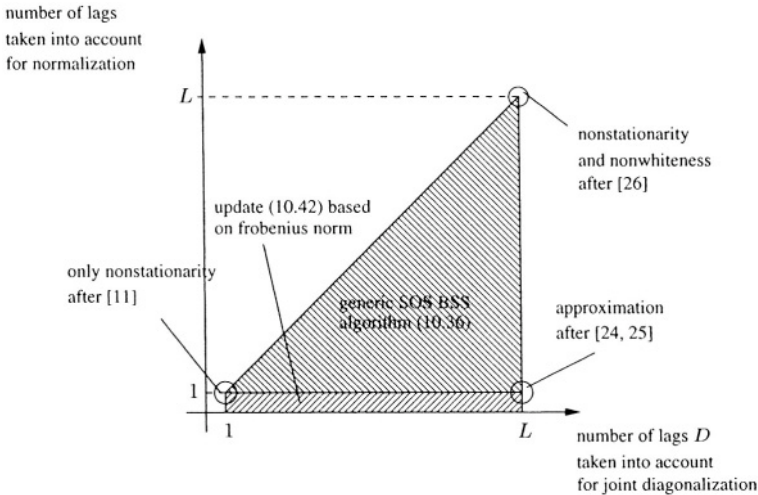
Figure 10.3 Overview of time-domain algorithms based on second-order statistics.
