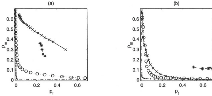
Figure 6.5 Receiver operating characteristic (ROC) (a) based on speech, (b) based on synthetic data. Double-talk detectors: Geigel ( \times ), cross-correlation ( \circ ), and normalized cross-correlation ( \cdot ). Region of operation for the threshold free two-path logic is indicated by (*). EBR = 0 dB and ENR = 30 dB.
