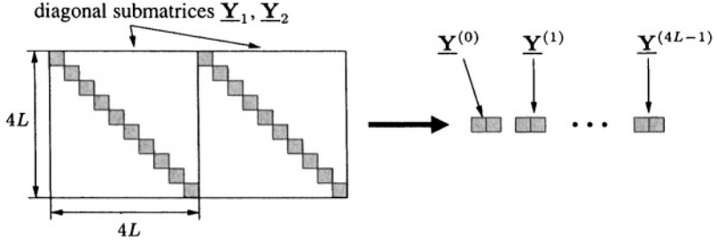
Figure 10.5 Illustration of bin-wise decomposition for the 2-channel case.
