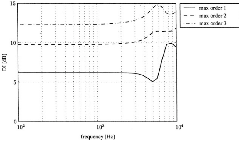
Figure 3.6 Maximum DI, allowing spherical harmonics up to order N , WNG is arbitrary.
