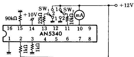
Test Circuit 1 ( I_{CC} , V_4 , 5, 6, 7, 8, 9, 11, 12, 16-1) ( V_{15-K(1)} , (2))
